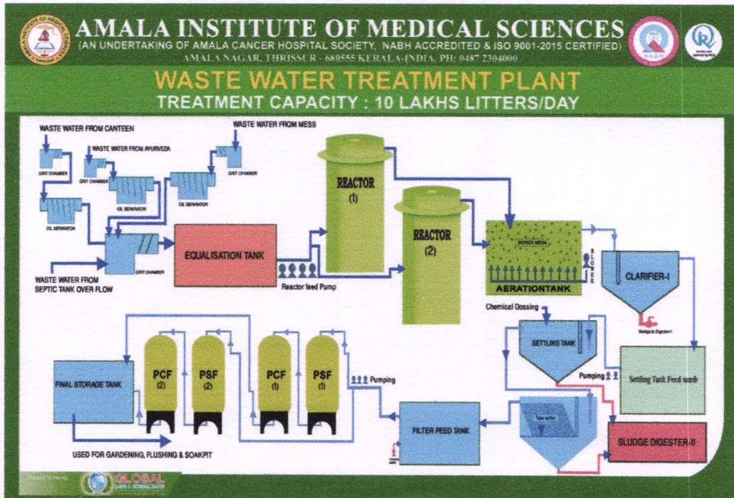
Flow chart showing the process of waste treatment plant
